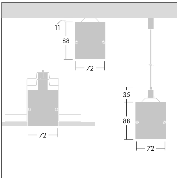
TLG_EQUL_M_surface_susepended_plasterboard.wmf
