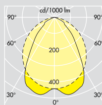
Indus XS mediumstrålende 2X49W T5 ULOR: 0% DLOR: 98% LOR: 98%
