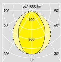
Indus RDx smalstrålende 2x49W T5 ULOR: 0% DLOR: 88% LOR: 88%
