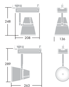
Graffiti M, track version
