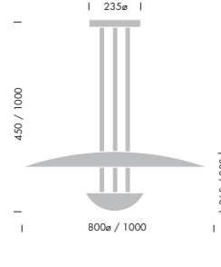
Uden uplight 800P/1000P
