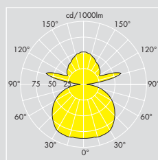
FATAMORGANA 1000/350 HFA 4 x 42W TC-TEL ULOR: 23% DLOR: 31% LOR: 54%
