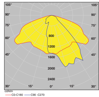
Dyana 60 LED Intensiv 60 stk 1,2W LED, 4200K, 5000lm
